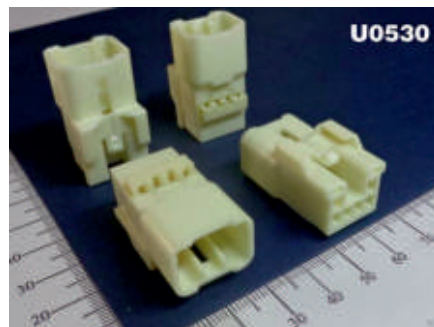
C-90 RT, 6 P M, With Lock
