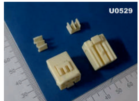
C-90 RT, 6 P F (with Secondary Lock)
