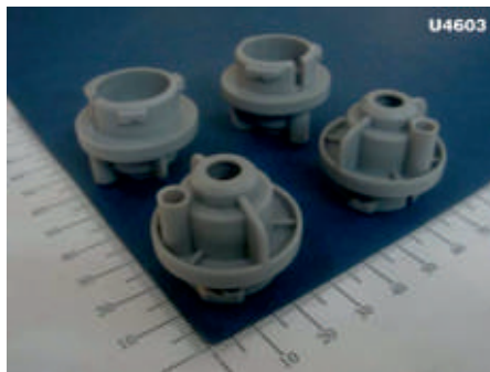
BULB HOLDER - 1490
