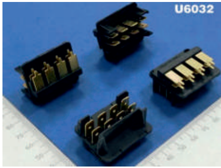
Cover-8-Pin-with-Terminal-Assy
