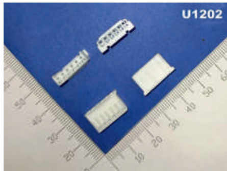
C-025, 6 P F, MR
