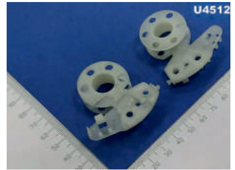
BOBBIN DIA-90
