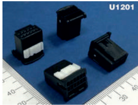
C-025, 12 P F, Black
