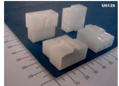
C-250, 6 P M, TL-Type, JEY
